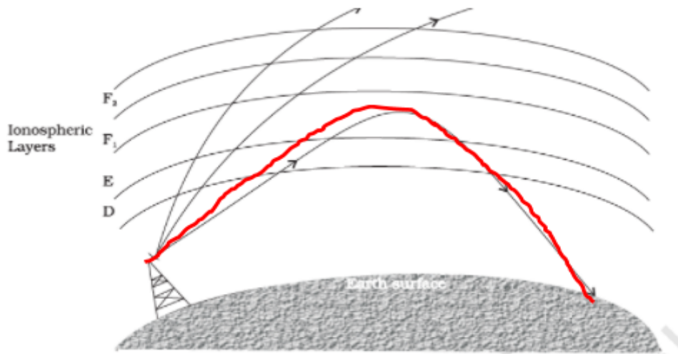
Marked in Red is Sky Wave Propagation
